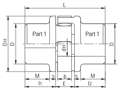
Serrated collar of polyurethane (Vulkollan) Shore hardness 92° Colour: natural
